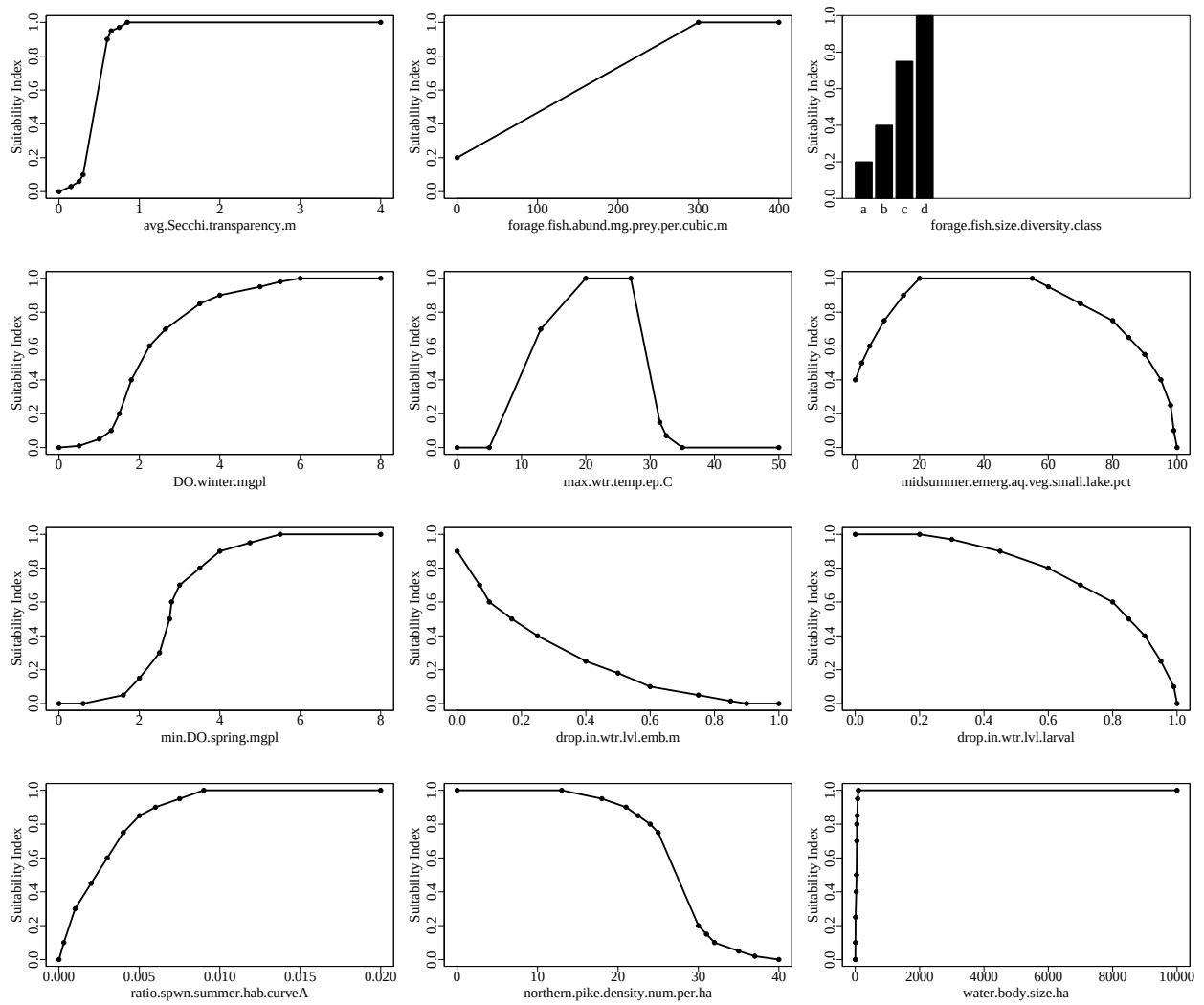
Figure 1. Suitability index graphs for variables included in the muskellungeSmallLakeSpwnVegCurveA model in ecoest.
